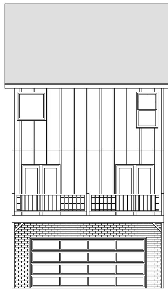
REAR ELEVATION 1/8"---1'-0"
