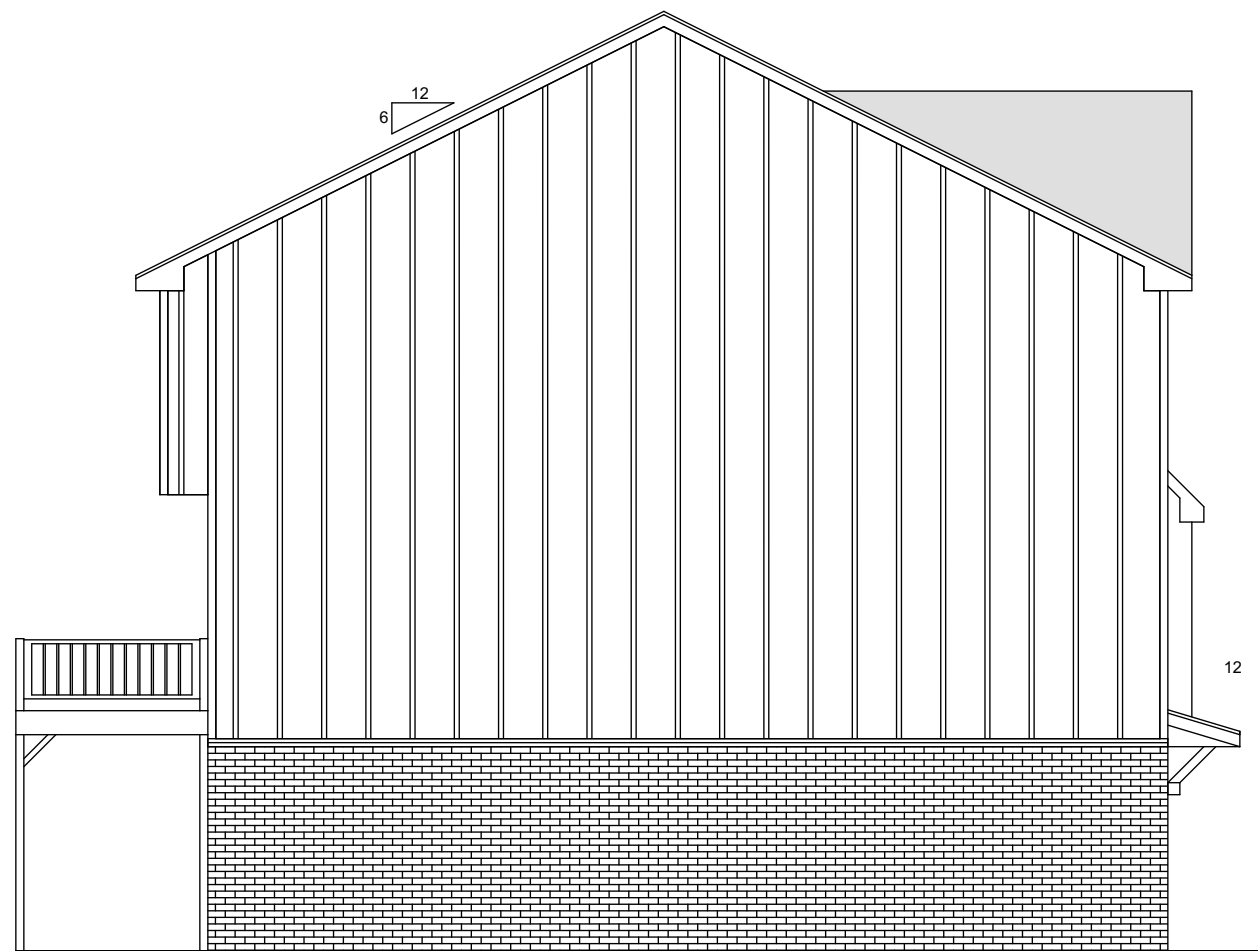
LEFT ELEVATION 1/8"---1'-0"
