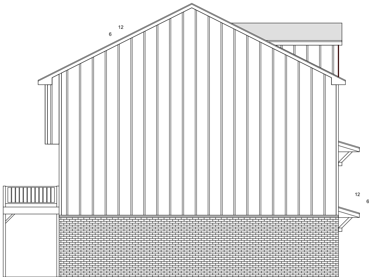
LEFT ELEVATION 1/8"---1'-0"
