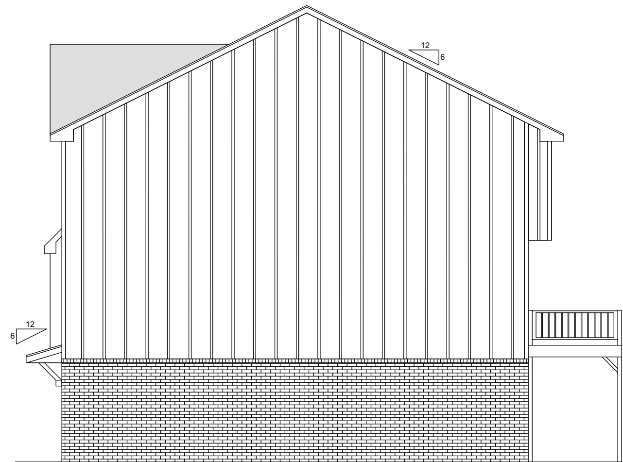
RIGHT ELEVATION 1/8"---1'-0"
