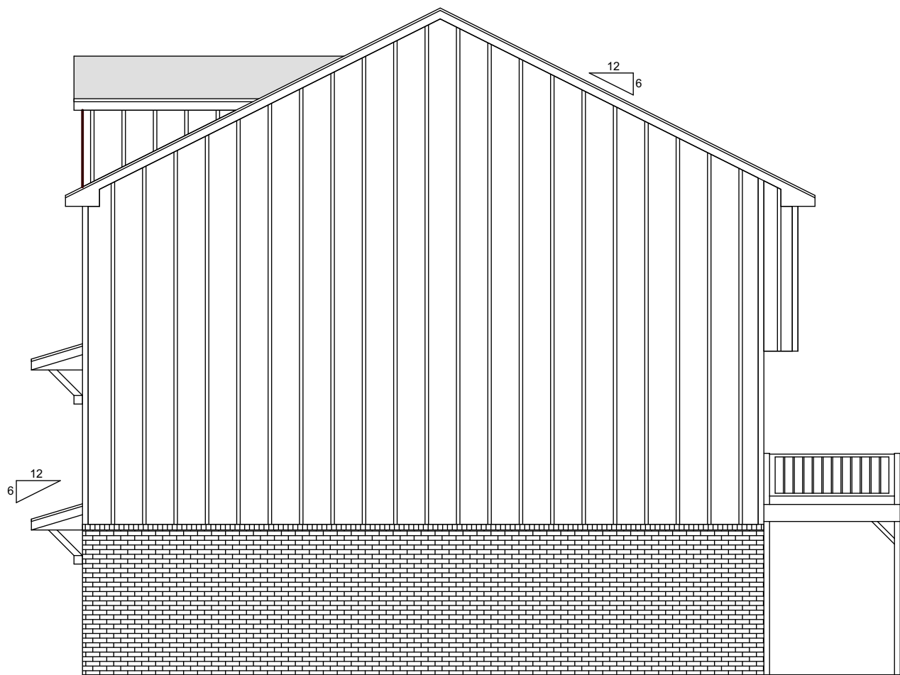
RIGHT ELEVATION 1/8"---1'-0"
