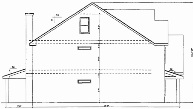
LEFT ELEVATION 1/8"-----1'-0"
