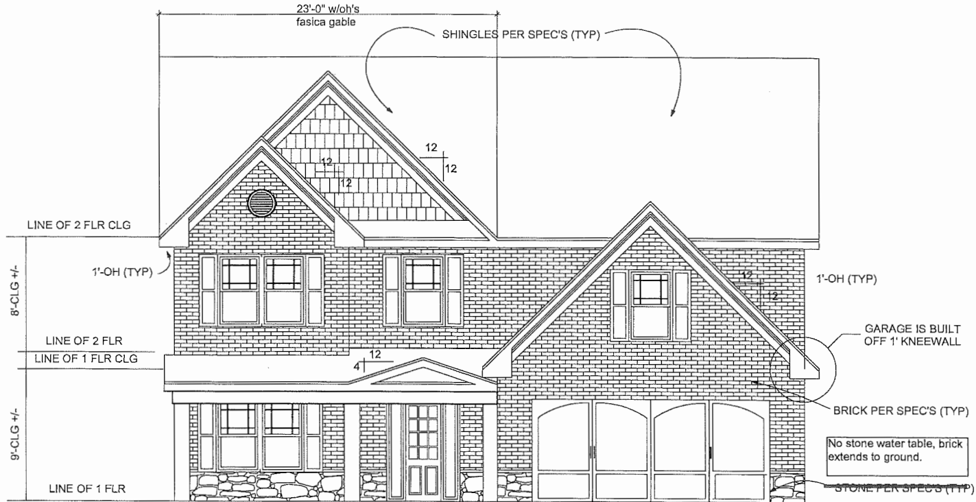
FRONT ELEVATION 1/4"-----1'-0"
