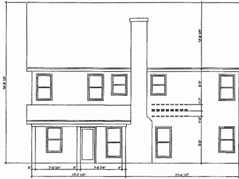
REAR ELEVATION 1/8"-----1'-0"
